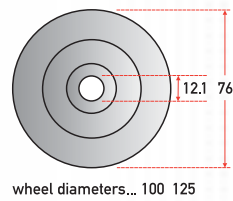
Single bolthole
